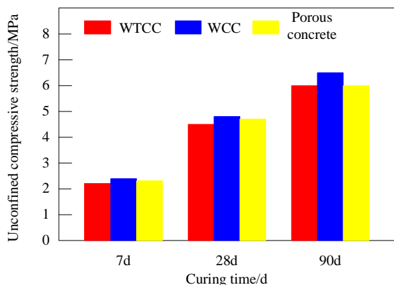
Figure 1. Compressive strength test chart.
