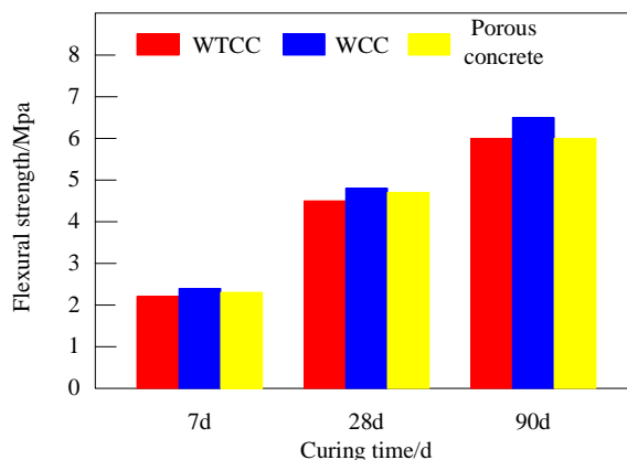
Figure 2. Bending strength test chart.
